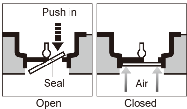
Valve diagram
