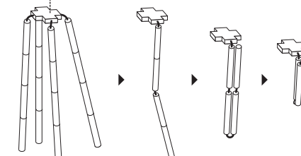
Fig. L Cross Socket
